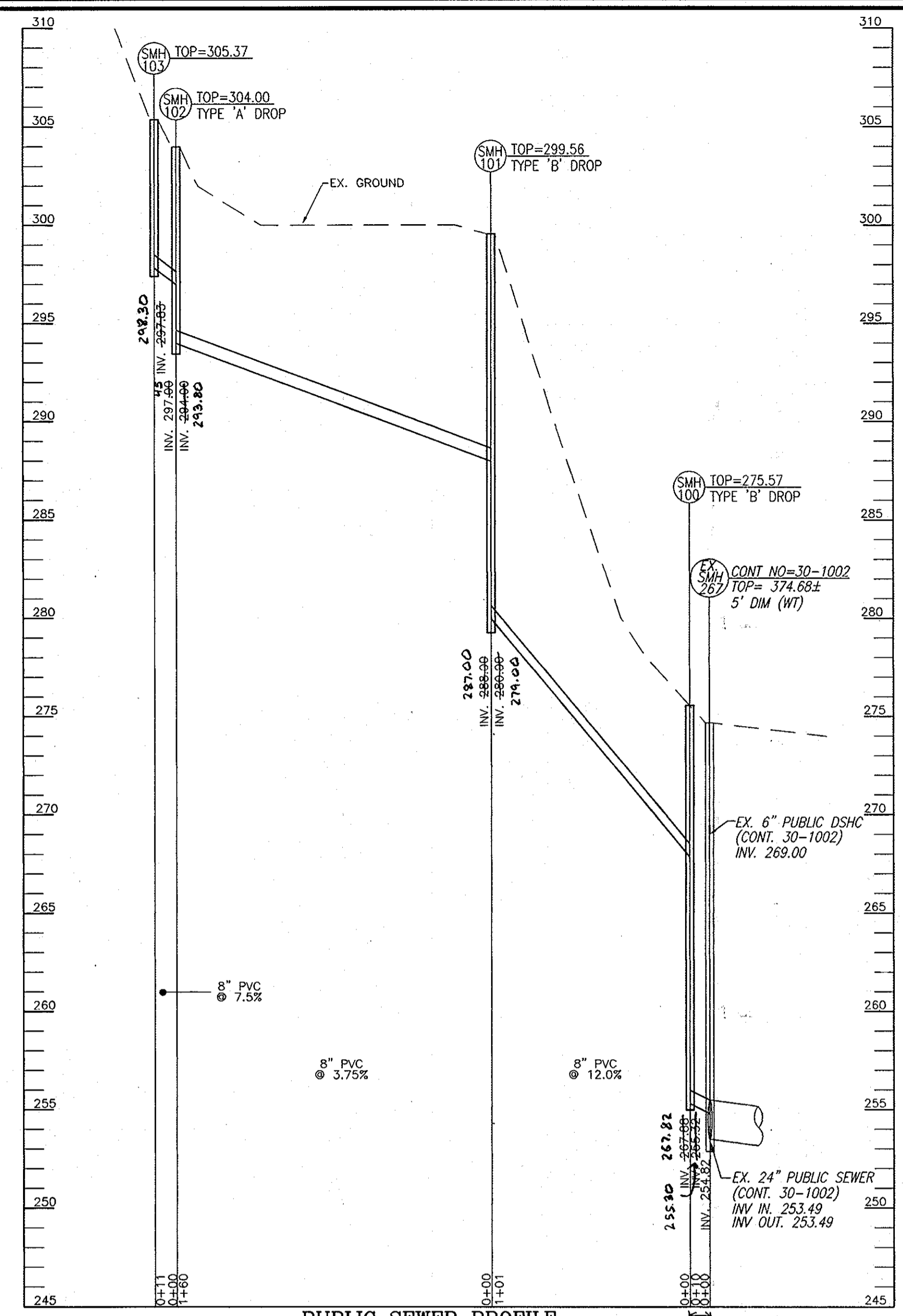
PUBLIC SEWER PROFILE SCALE: HORIZONTAL - 1"=50' VERTICAL - 1"=5'
