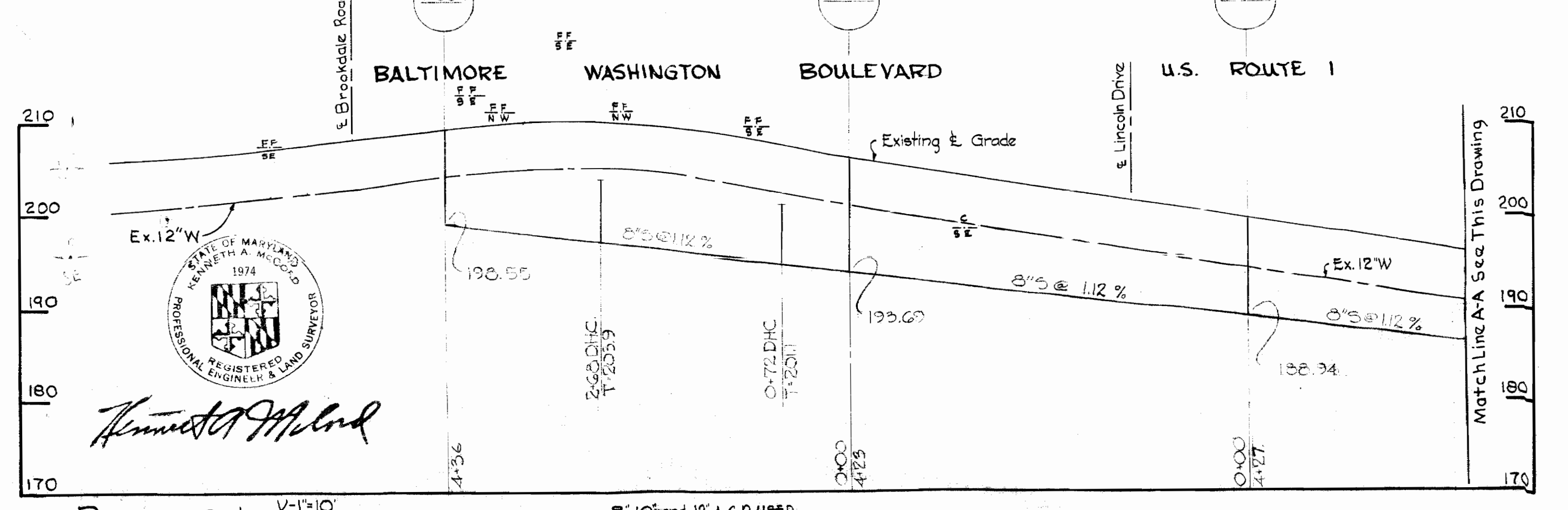
PROFILE Scale: V-1"=10' H-1"=100'
