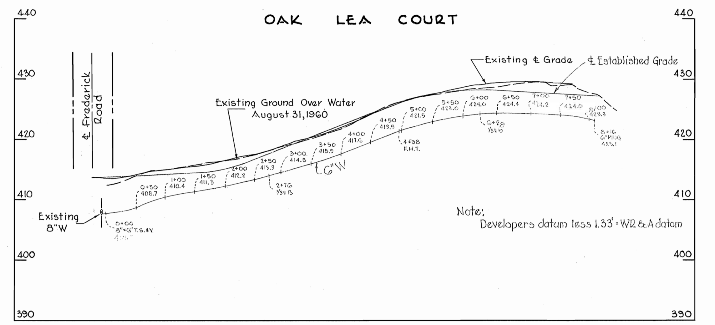
PROFILE Horiz. 1"=100' Scale: Vert. 1"=10'
