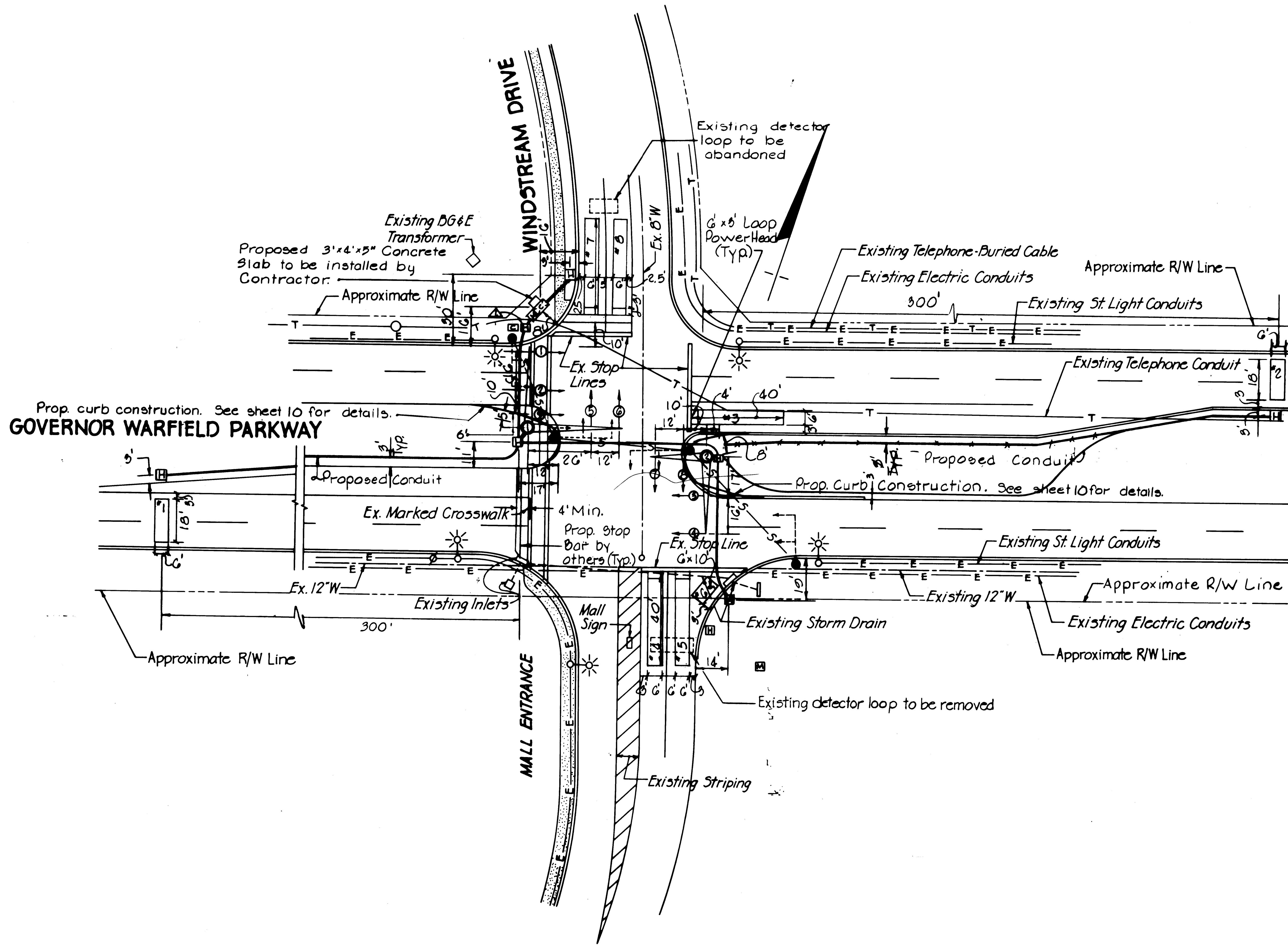
PLAN Scale 1" = 30'
