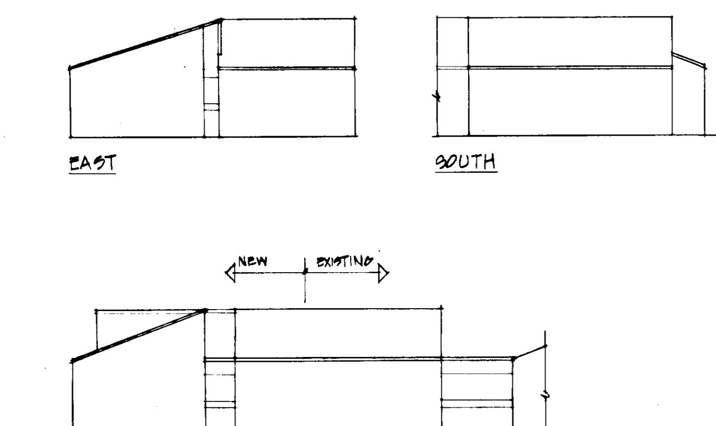
NORTH SCHEMATIC ELEVATIONS OF PROPOSED NEW RACQUETBALL COURTS SCALE: 1/4"=1'-0"
