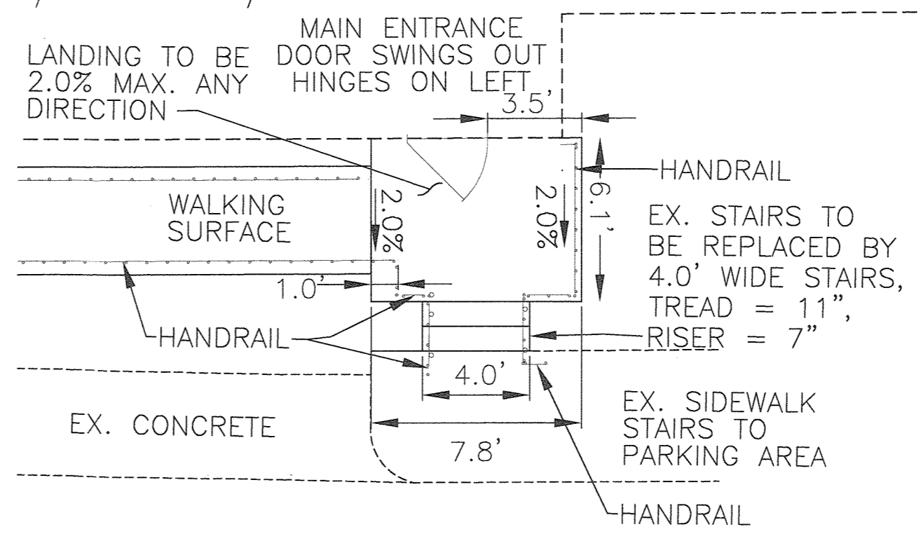
LANDING/ENTRANCE DETAIL
