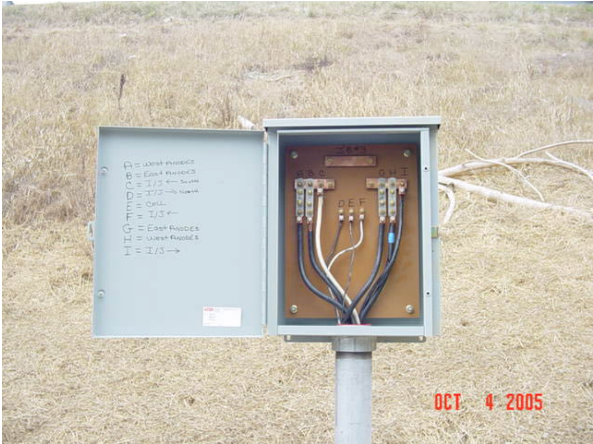
Figure 8 – Test Station 3
