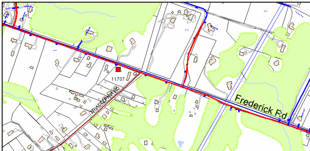
Figure 74 - Location of the Impressed Current Rectifier ST11
