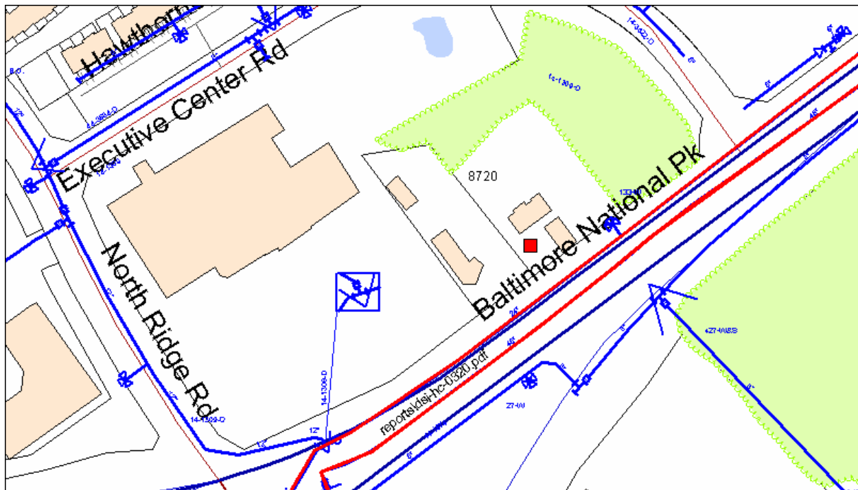
Figure 66 - Location of the Impressed Current Rectifier ST7
