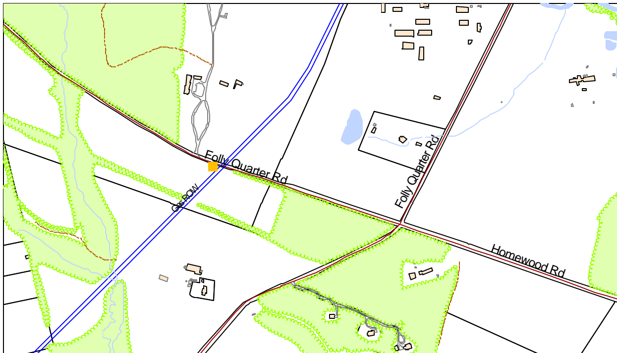
Figure 39 - Location of Impressed Current Rectifier TR4
