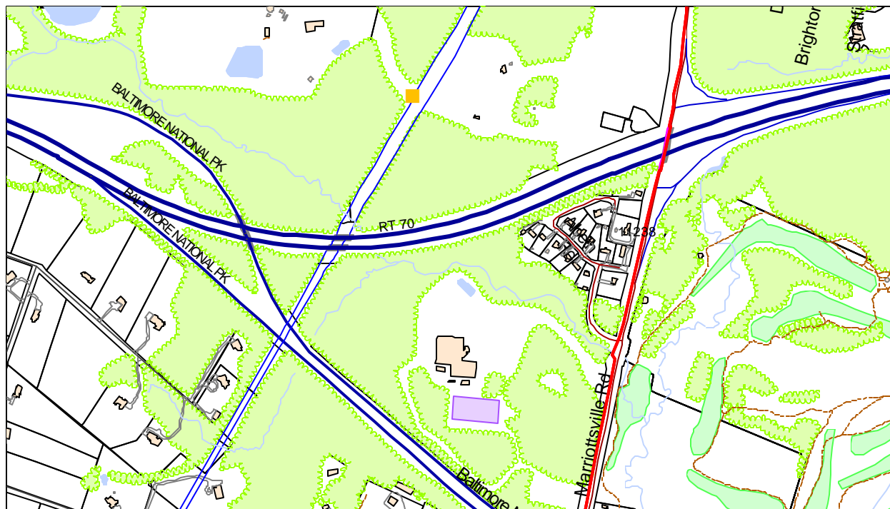
Figure 35 - Location of Impressed Current Rectifier TR2
