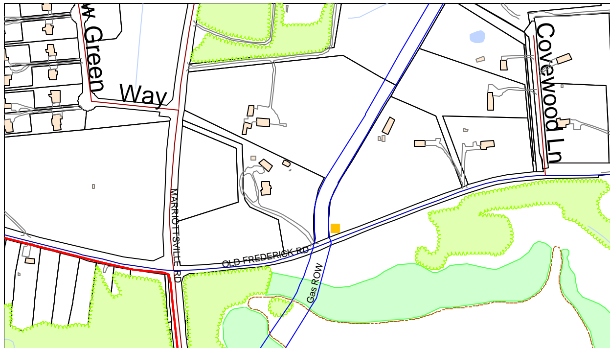
Figure 33 - Location of Impressed Current Rectifier TR1
