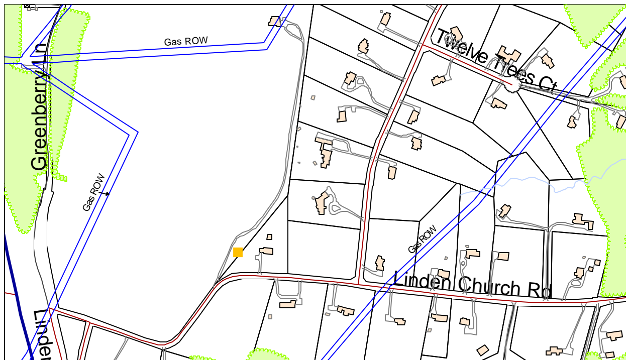
Figure 43 - Location of Impressed Current Rectifier CMB2
