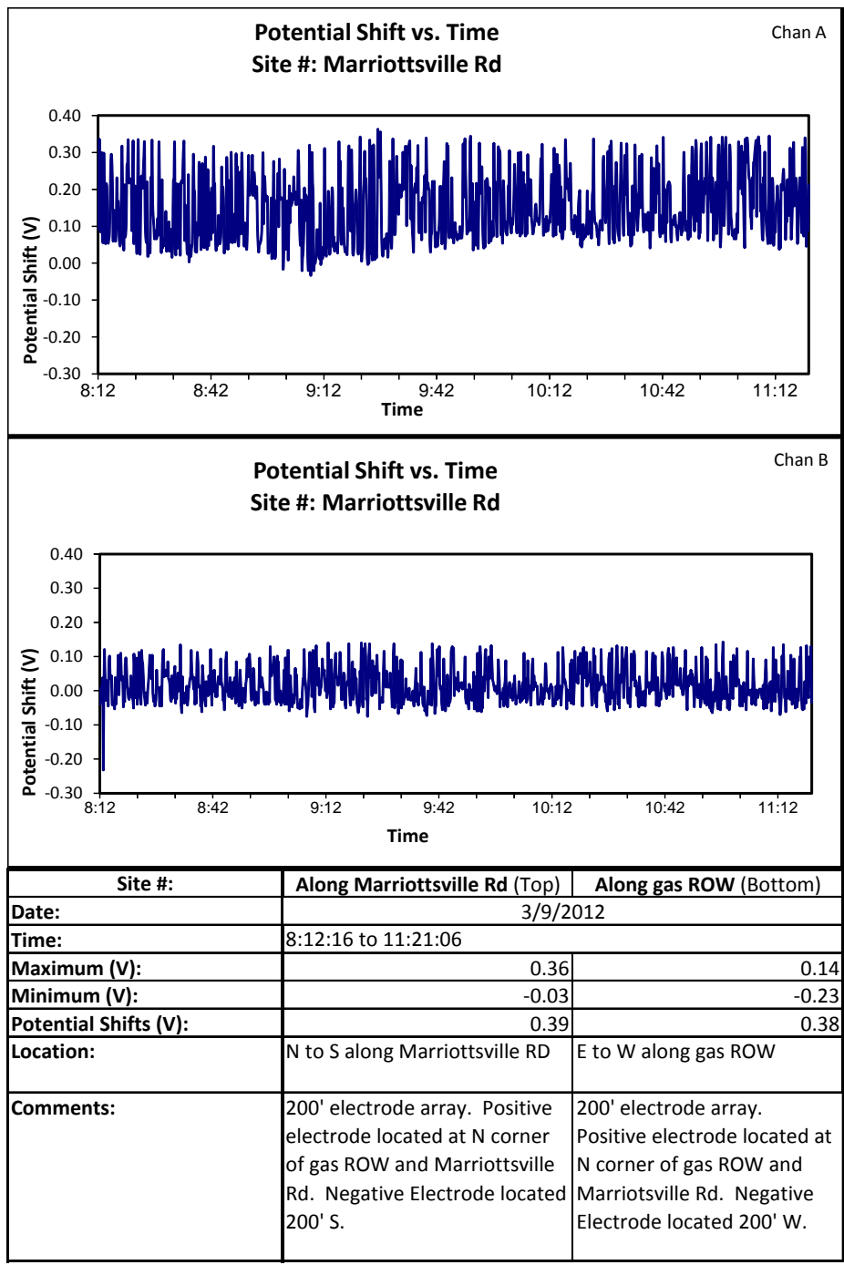
Figure 45 - Results of Stray Current Test #4 on Marriottsville Rd
