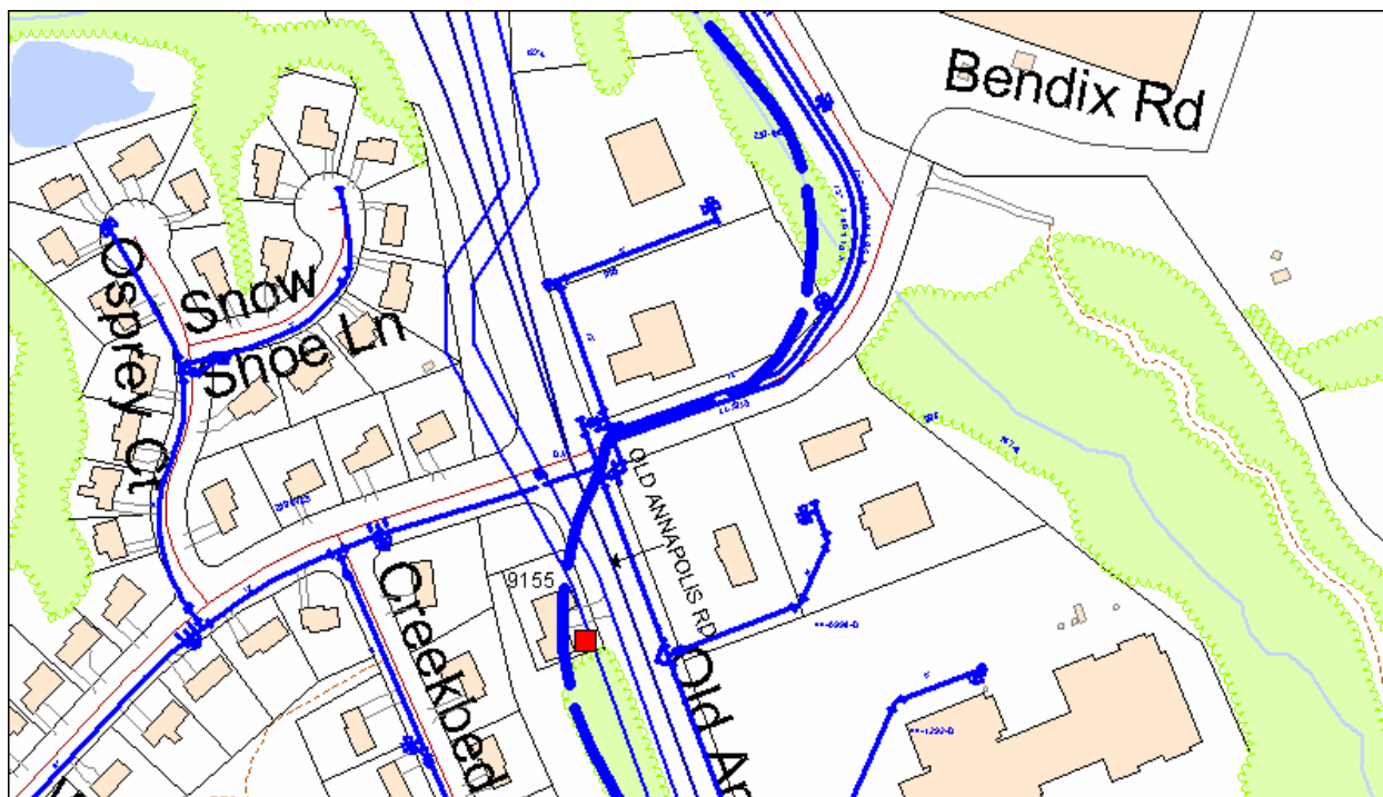
Figure 64 - Location of the Impressed Current Rectifier ST6
