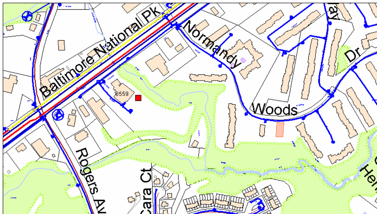
Figure 60 - Location of the Impressed Current Rectifier ST4
