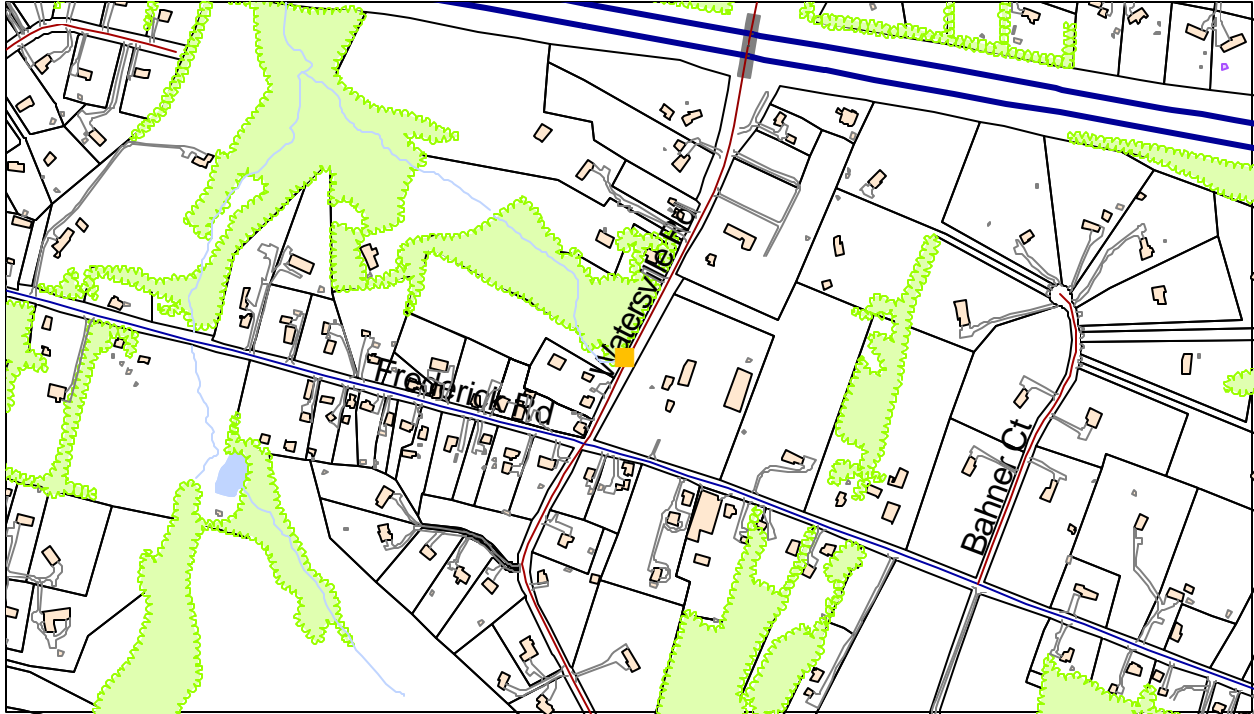
Figure 9 - Location of Impressed Current Rectifier BGE2
