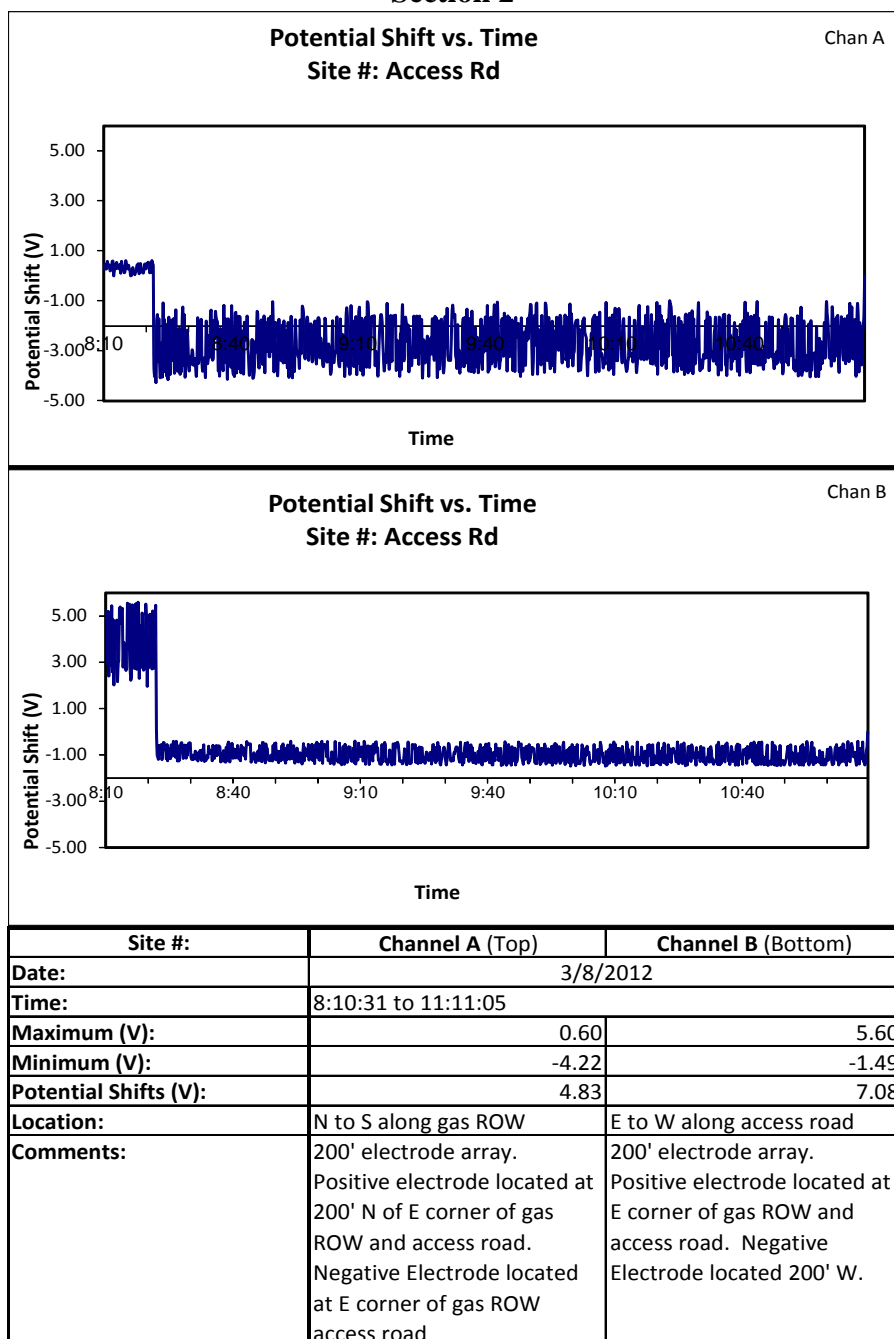
Figure 44 - Results of Stray Current Test #3 on the Access Road near Alpha Ridge Landfill
