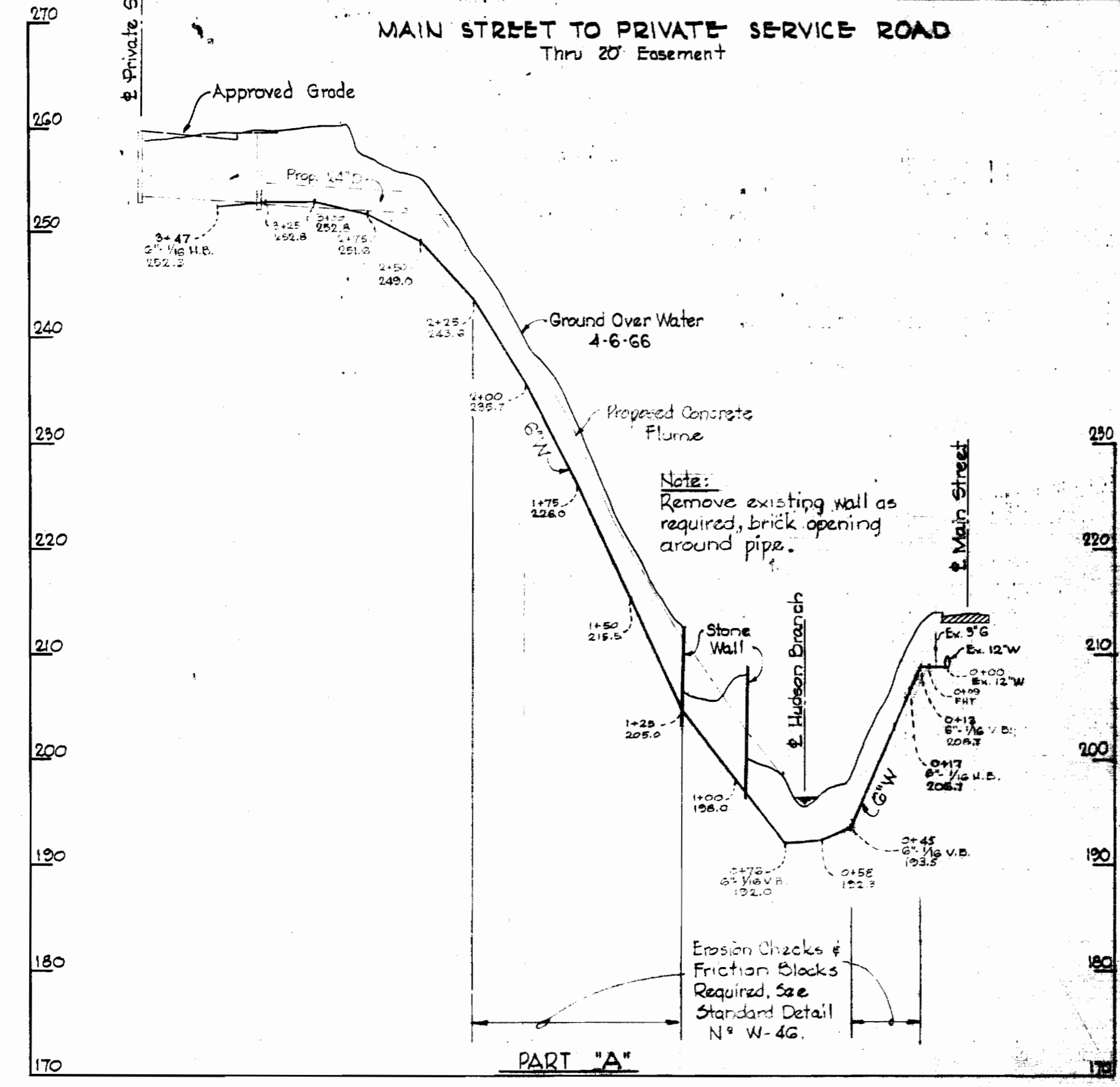
PROFILE Scale: Hor. - 1" = 50' Vert. - 1" = 10'
