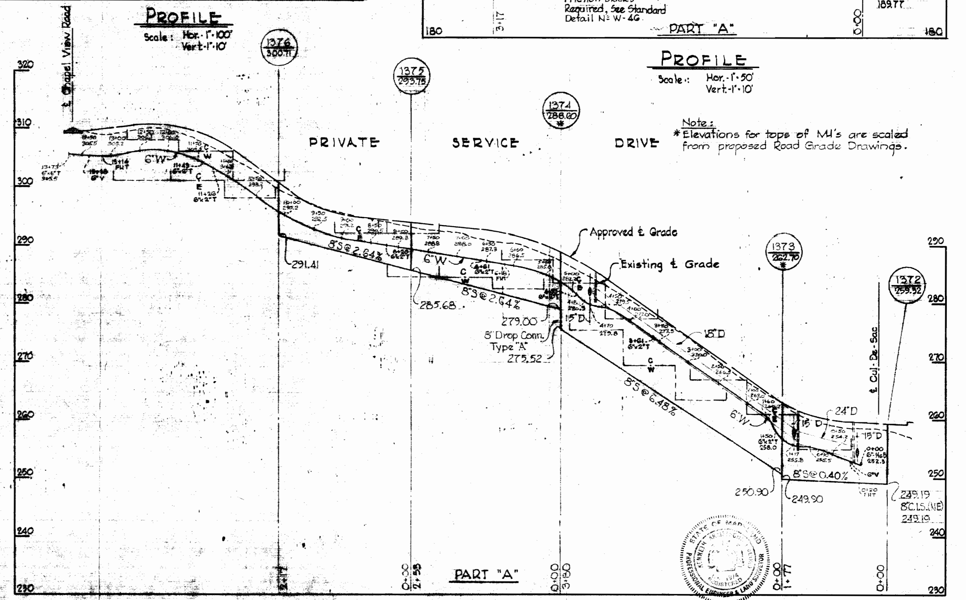
PROFILE Scale: Hor. - 1" = 100' Vert. - 1" = 10'
