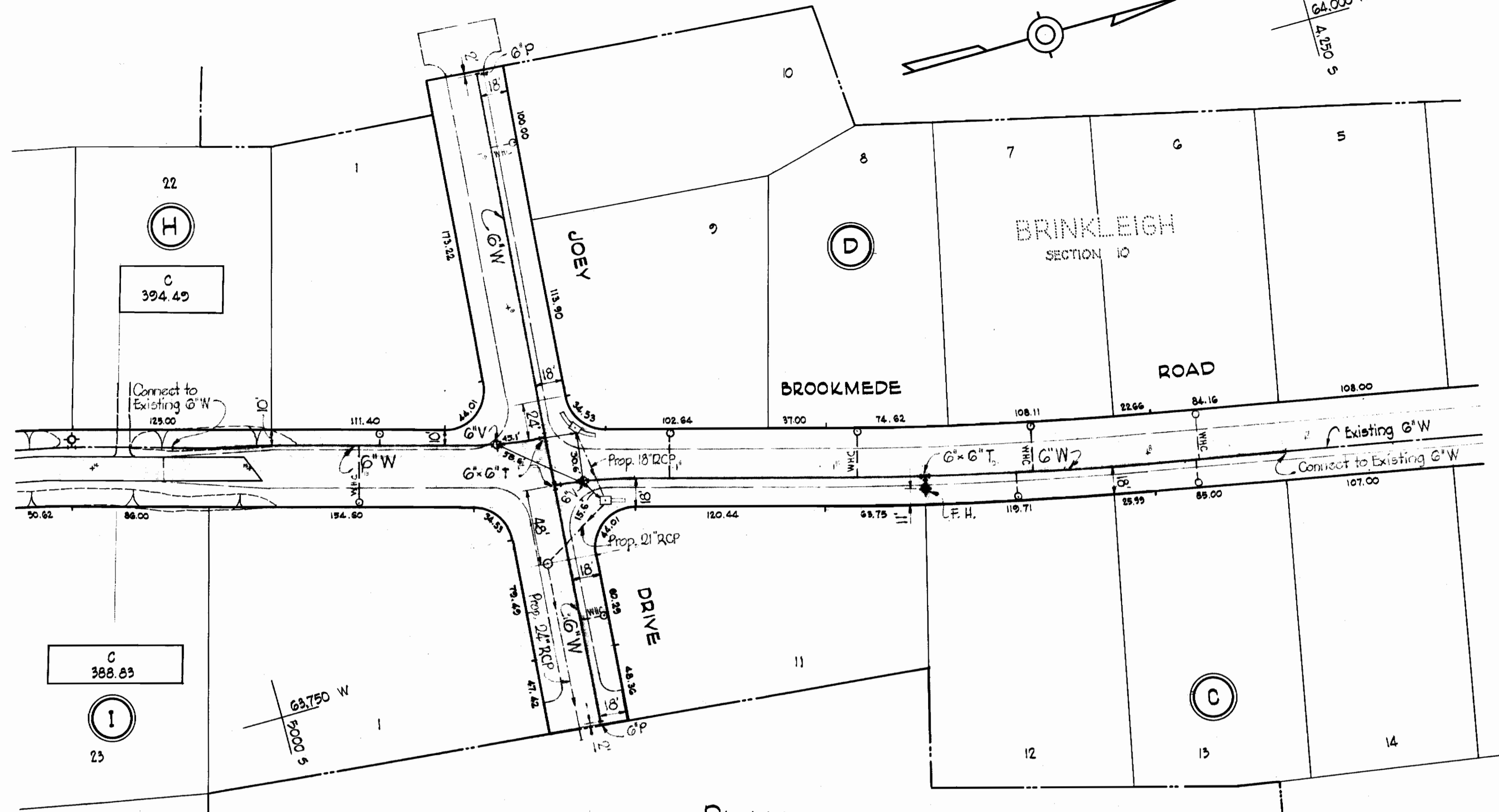
PLAN Scale: 1"=50'
