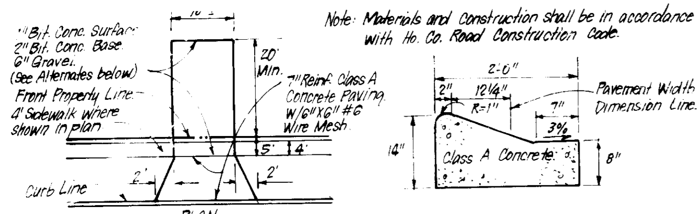
DRIVEWAY ABUTTING MODIFIED CURB & GUTTER*
