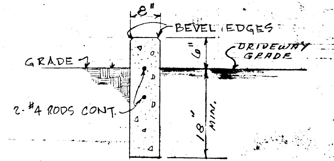
TYPICAL SECTION THRU PROPERTY LINE AND INTERIOR CURBS
