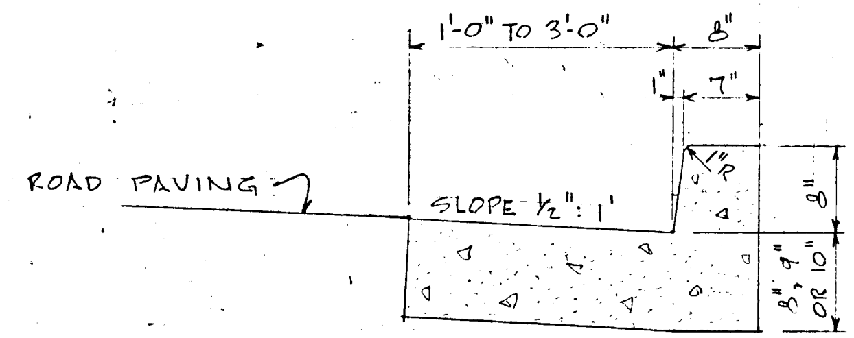
SECTION THRU EXISTING CURB & GUTTER @ HARPER'S FARM ROAD
