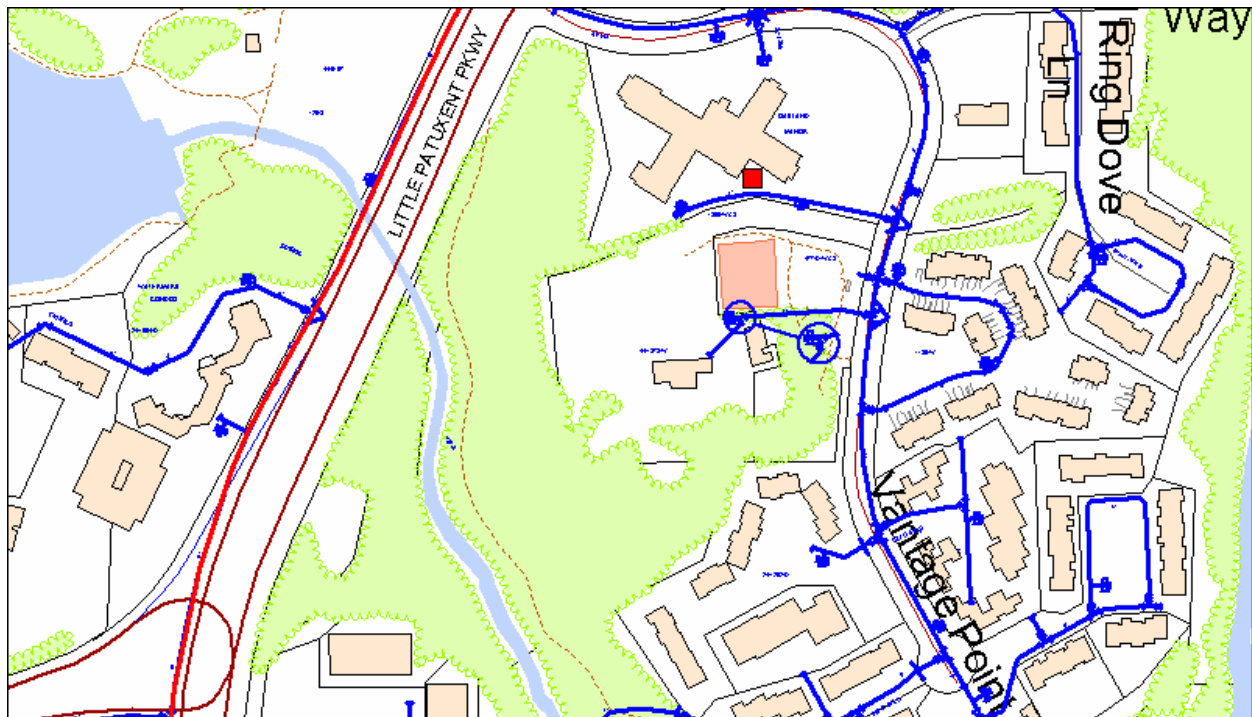
Figure 80 - Location of the Impressed Current Rectifier ST14
