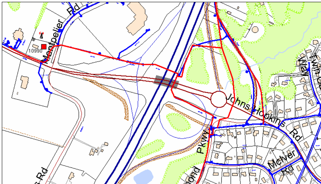
Figure 58 - Location of the Impressed Current Rectifier ST3
