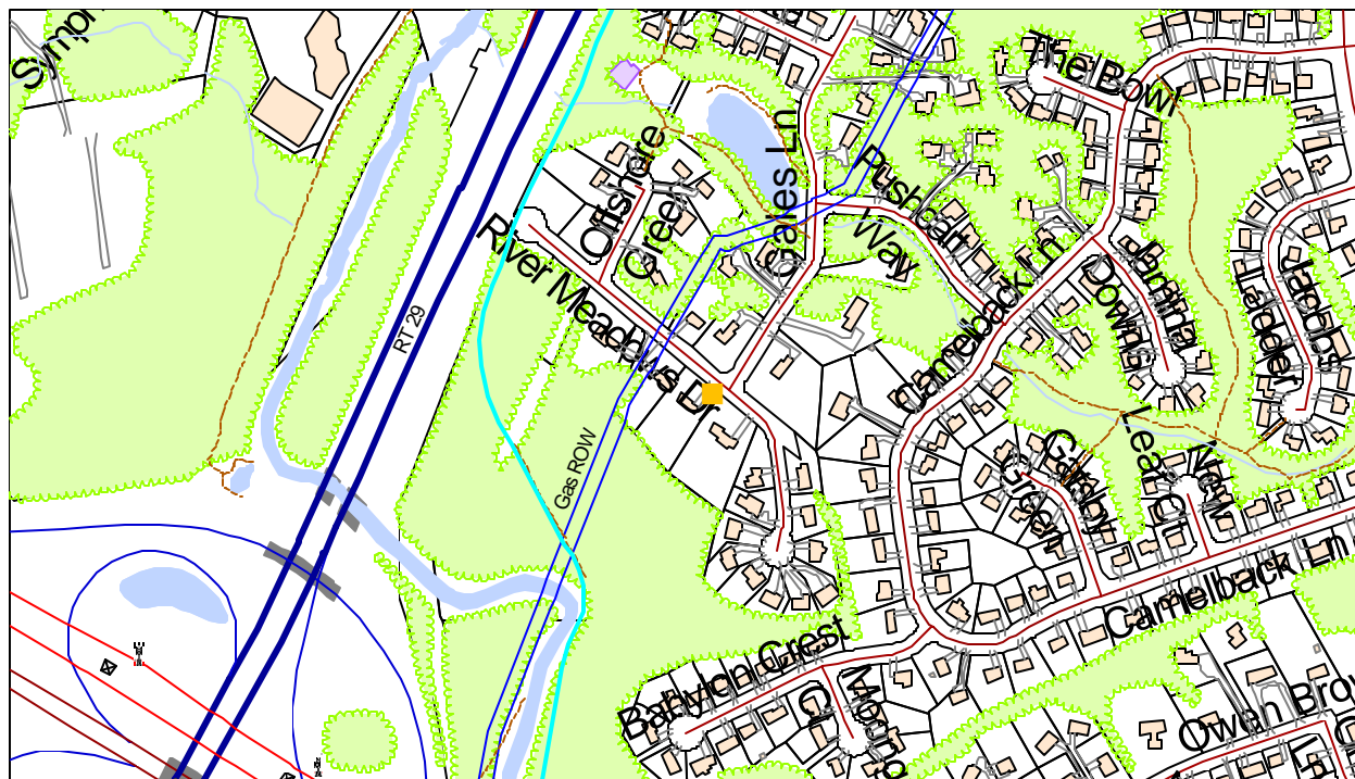
Figure 48 - Location of Impressed Current Rectifier COL2
