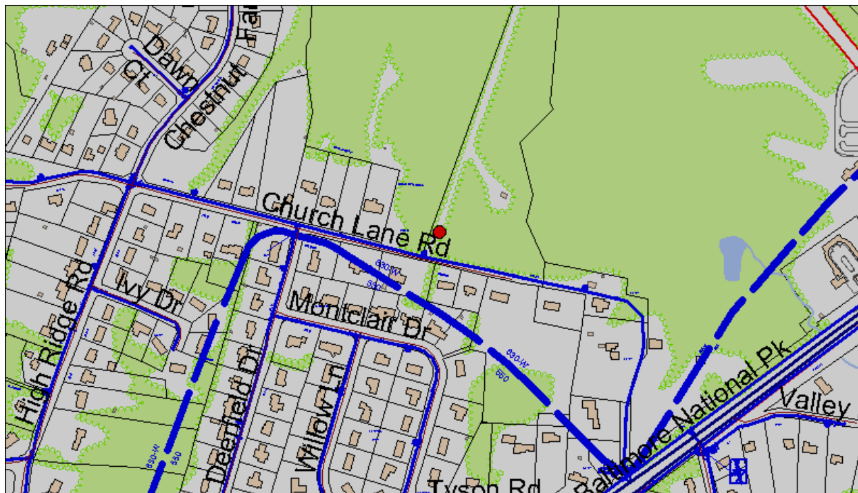
Figure 86 - Location of the stray current testing location for the Chestnut Hill substation
