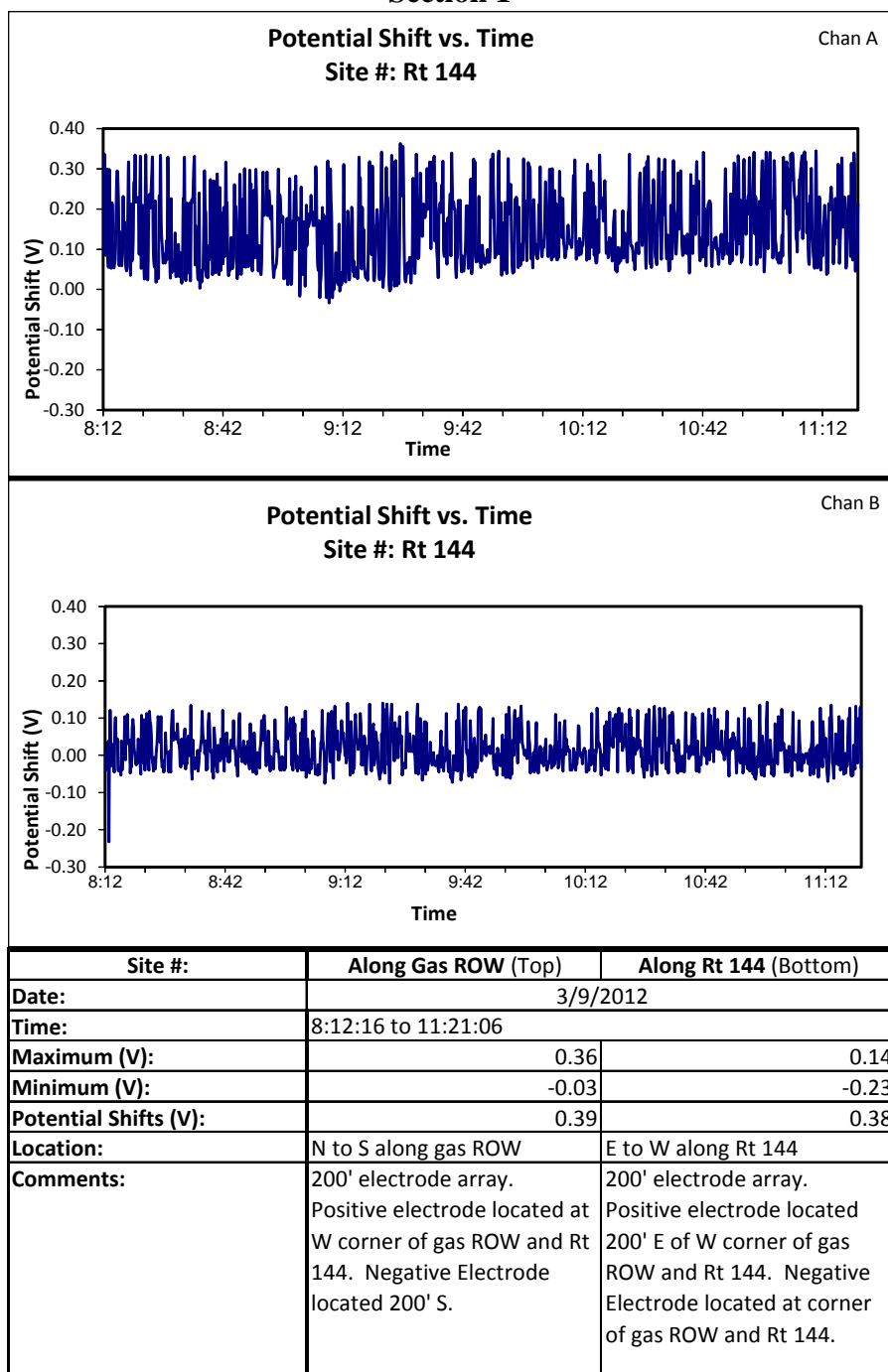
Figure 42 – Results of Stray Current Test #1 on Rt 144
