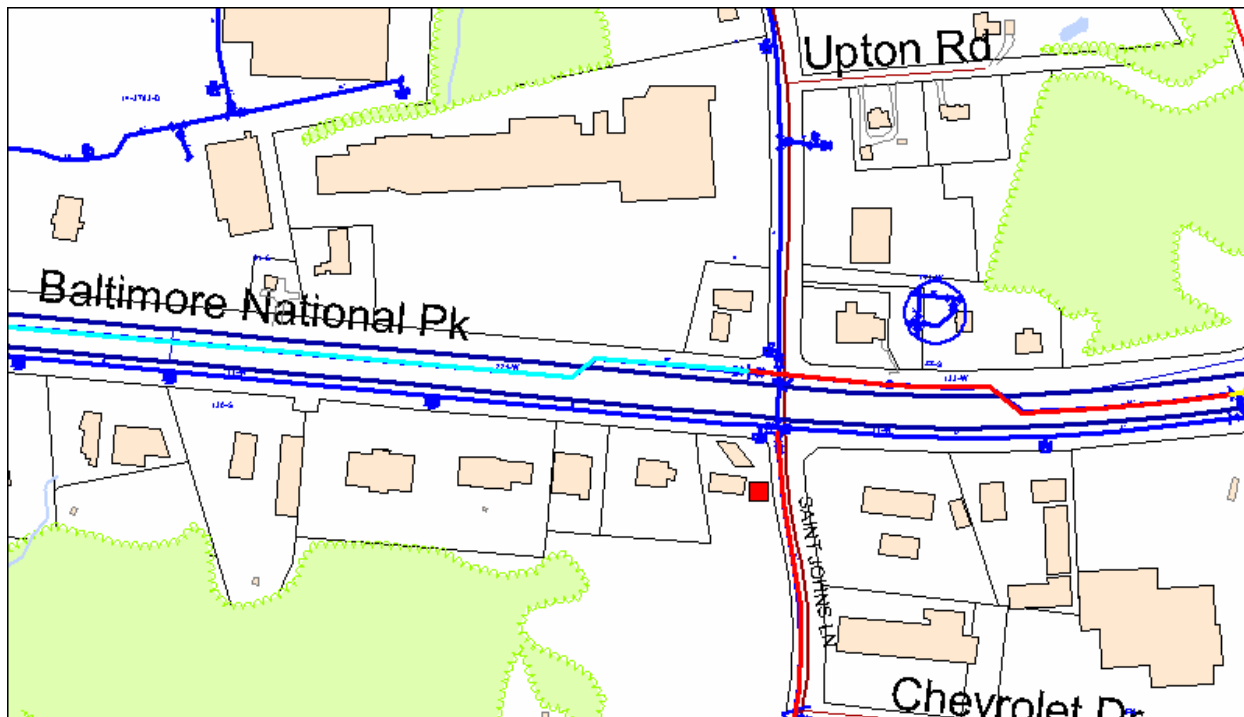
Figure 70 - Location of the Impressed Current Rectifier ST9
