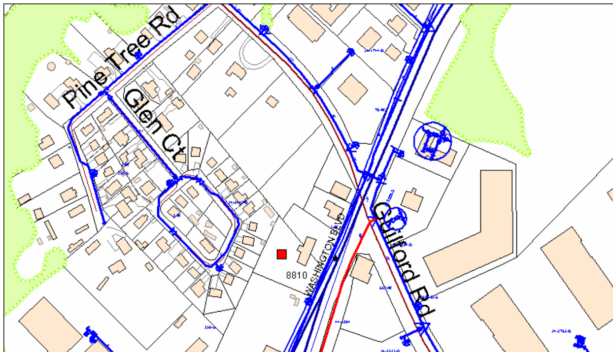
Figure 62 - Location of the Impressed Current Rectifier ST5
