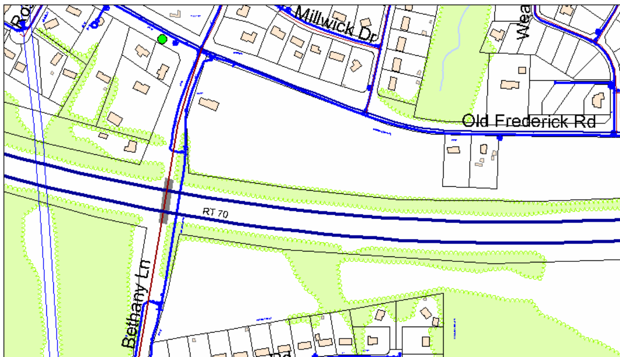
Figure 116 – Stray current location near Bethany Lane and Route 99
