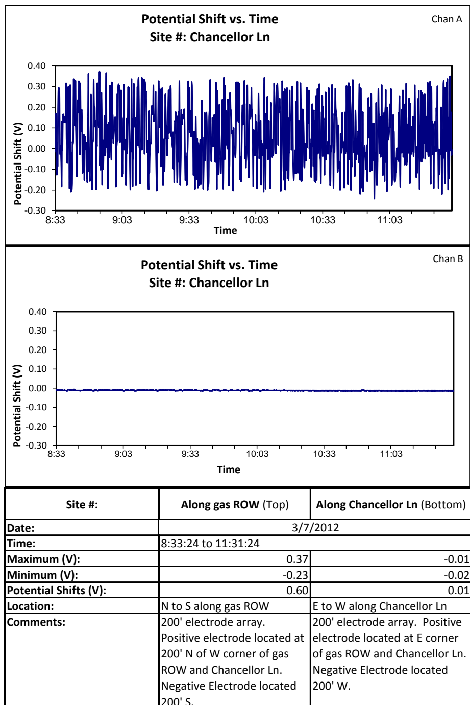
Figure 43 - Results of Stray Current Test #2 on Chancellor Ln
